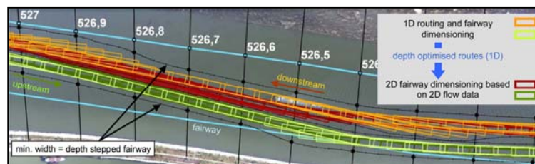
Swept areas from PeTra1D and PeTra2D calculations of vessels driving upstream and downstream and additional safety distances, resulting in the "Depth stepped fairway".
